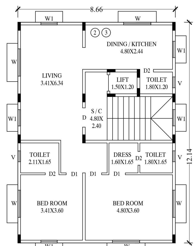
PROPOSED TYPICAL FIRST & SECOND FLOOR PLAN
