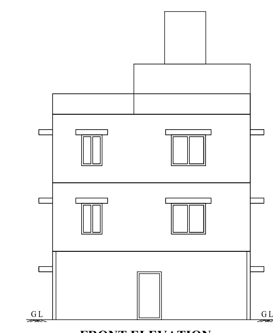
FRONT ELEVATION
